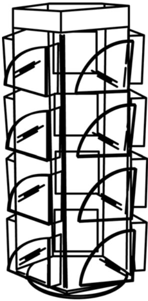
CT-001 CD Counter Spinner Unit. Made from clear acrylic with injection moulded pockets. Holds 60 CD's. Optional printed header section. Overall size (mm) 350w 655h 350d.
